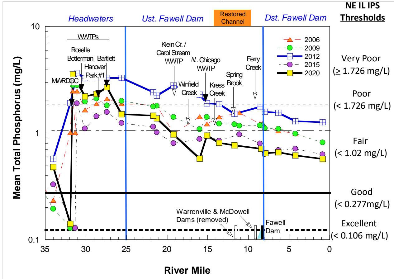
Figure 36. West Branch DuPage River mean instream TP concentrations for Basin Assessment years 2006, 2009, 2012, 2015, and 2020.
